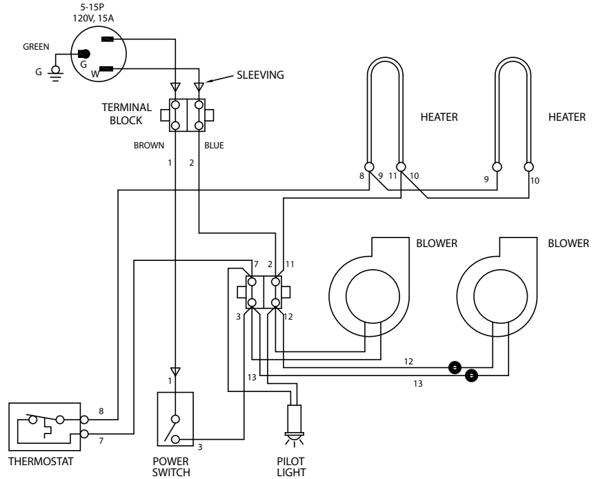
DIAGRAM FOR 120V UNITS
