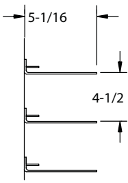
DETAIL OF PAN SLIDE
