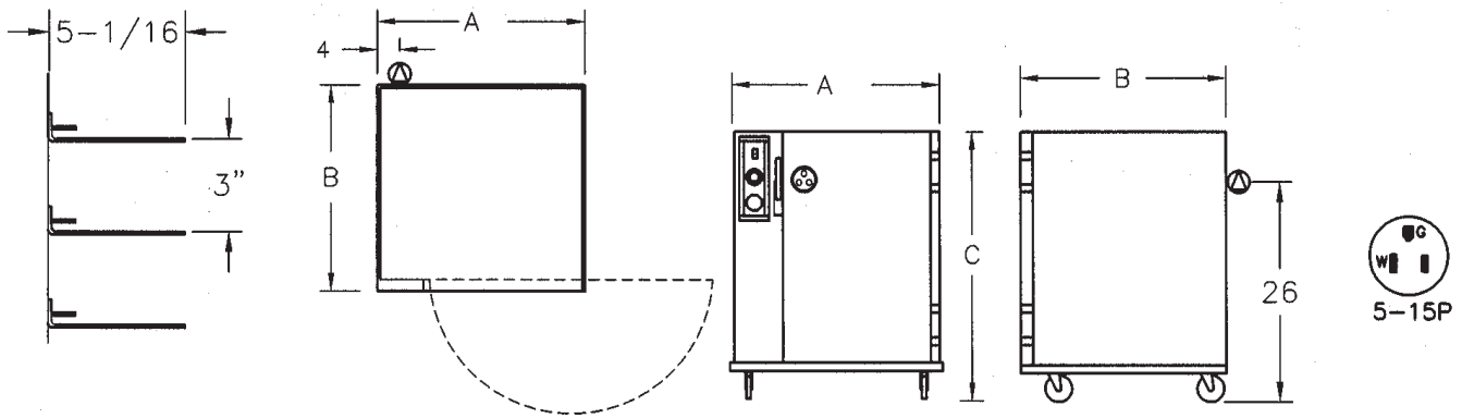
DETAIL OF PAN SLIDE
