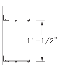
DETAIL OF PAN SLIDE
