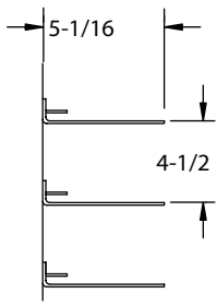
DETAIL OF PAN SLIDE
