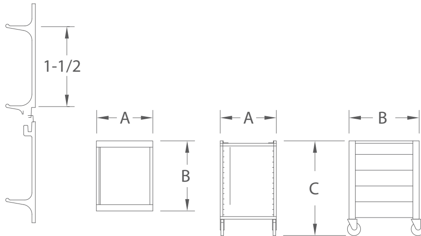
DETAIL OF PAN SLIDE
