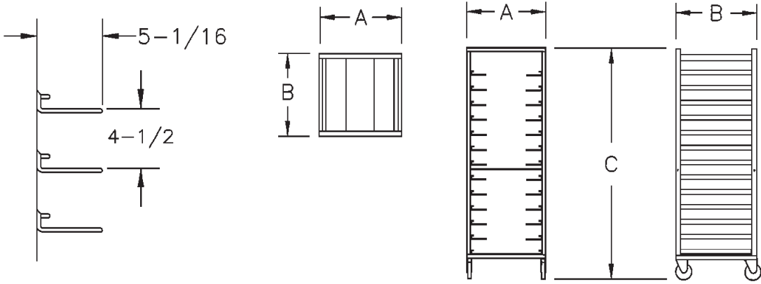
DETAIL OF PAN SLIDES
